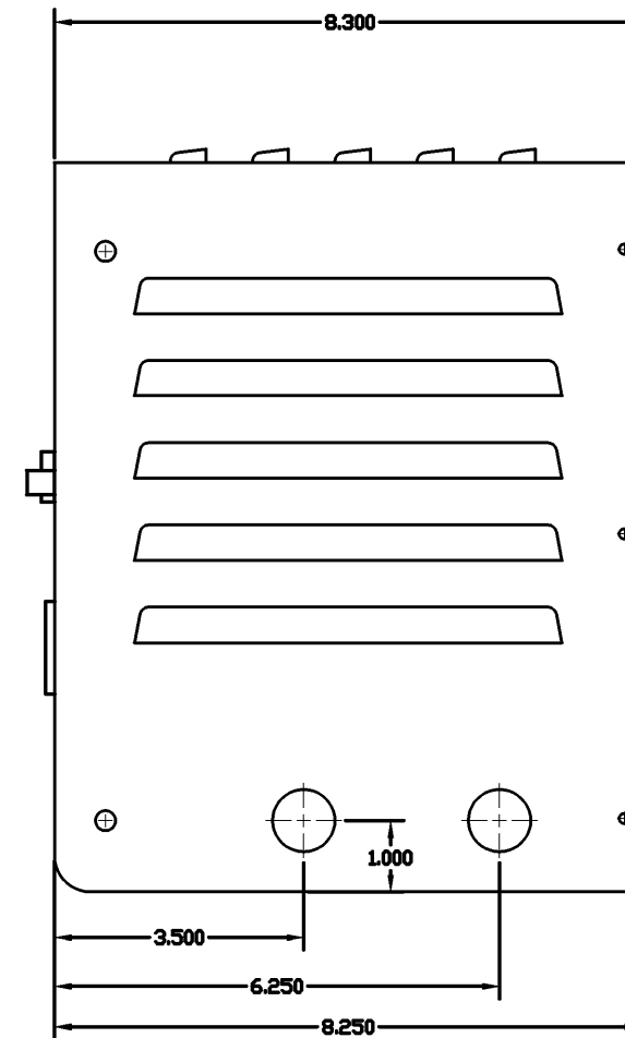
RIGHT SIDE
